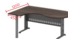
SUPERIOR COMPACT TABLE (L) QL 66-M 1800W x 900 x 1200 x 450D x 750H
