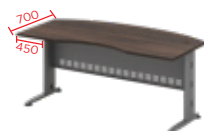
EXECUTIVE TABLE QMB 55 1800W x 900D x 750H
